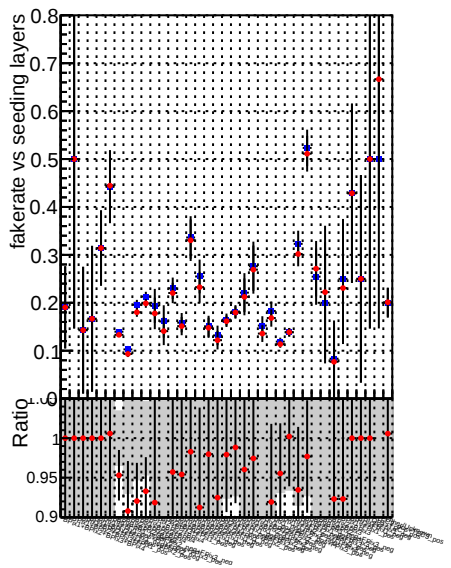
Fake rate vs. —•— DQM V0001 R000000001 Global mkFit 100stable —•— DQM V0001 R000000001 Global mkFit CAND100stable
