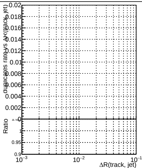
—●— DQM_V0001_R000000001_Global_mkFit_100stable —●— DQM_V0001_R000000001_Global_mkFit_CAND100stable
