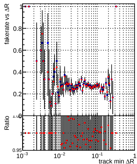
—●— DQM_V0001_R000000001_Global_mkFit_100stable —●— DQM_V0001_R000000001_Global_mkFit_CAND100stable
