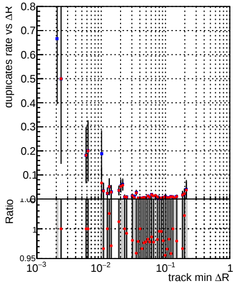
—●— DQM_V0001_R000000001_Global_mkFit_100stable —●— DQM_V0001_R000000001_Global_mkFit_CAND100stable
