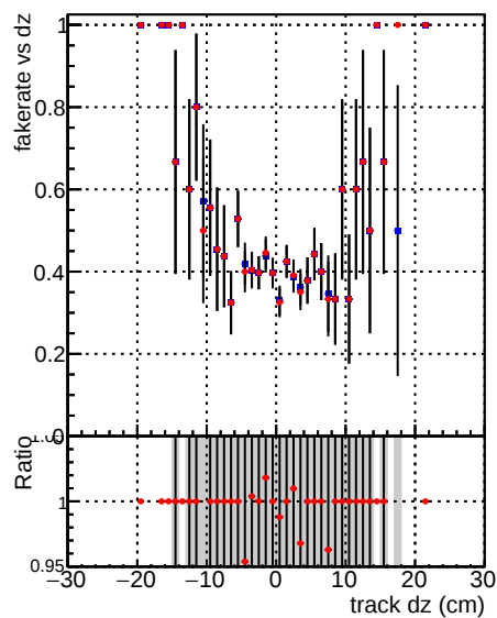
Fake rate vs dz DQM V0001_R000000001 Global mkFit 100stable DQM V0001_R000000001 Global mkFit CAND100stable
