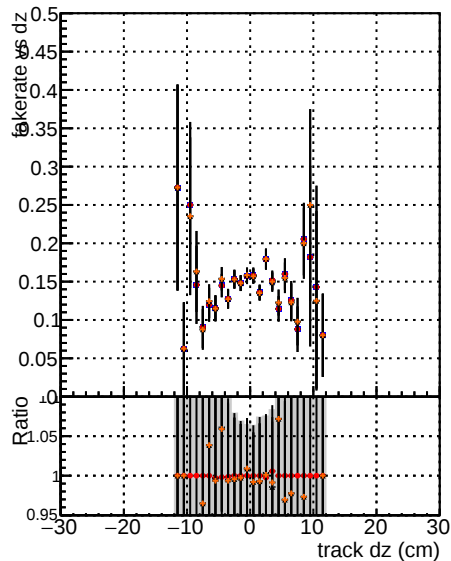
Fake rate vs d DQM V0001 B00000000001 Global mkFit original DQM V0001 B00000000001 Global mkFit pass DQM V0001 R00000000001 Global mkFit new
