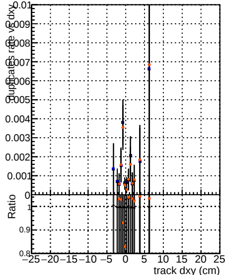
Legend for all plots: DGM v0001 (black) DGM v0001 (blue) DGM v0001 (orange) Global (red) mkFit original (green) mkFit new (purple)
