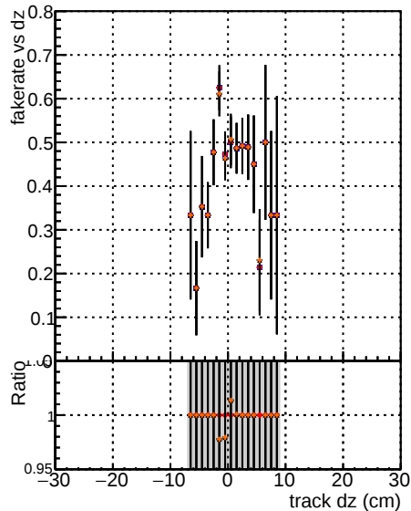
Fake rate vs d DOM V0001 B0000000001 Global mkFit original DOM V0001 B0000000001 Global mkFit post DOM V0001 R0000000001 Global mkFit post DOM V0001 R0000000001 Global mkFit new
