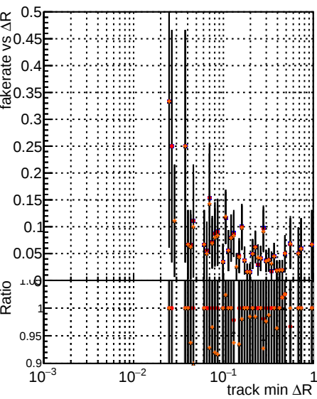
Fake rate vs \Delta R(\text{track}, \text{jet}) Legend: Global (black) Global mkFit (blue) Global mkFit pless (red) Global mkFit new (orange)
