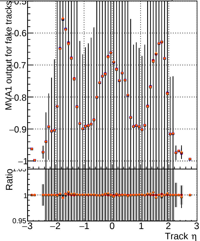
MVA1 of associated tracks (recoToSim) vs. track \eta Legend: Track Type Model Global mkFit Original Associated DQM_V0001_R0000000001 Global mkFit original Associated DQM_V0001_R0000000001 Global mkFit plebs Associated DQM_V0001_R0000000001 Global mkFit hptt Associated DQM_V0001_R0000000001 Global mkFit new
