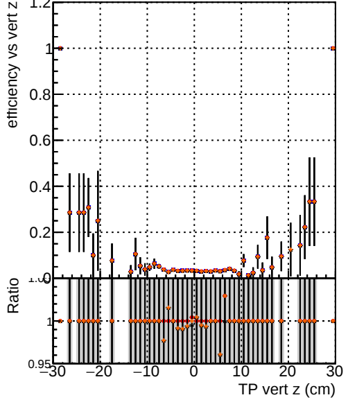
—●— DQM_V0001_R0000000001 Global mkFit_original —●— DQM_V0001_R0000000001 Global mkFit_pless —●— DQM_V0001_R0000000001 Global mkFit_hptt —●— DQM_V0001_R0000000001 Global mkFit_new
