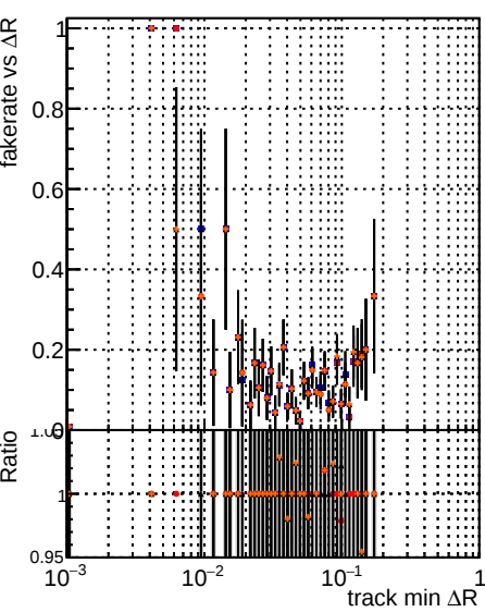
Fake rate vs \Delta R(\text{track, jet}) Legend: Global mktFit mktFit+plecs mktFit+new
