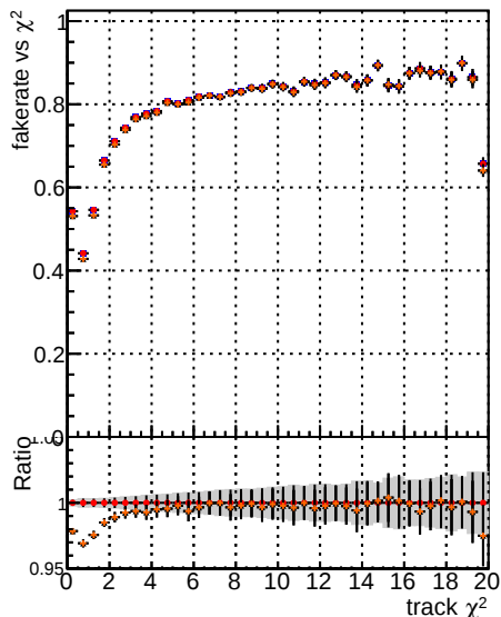
Fake rate vs. DOM V0001 B00000000001 Global mkFit original B00000000001
