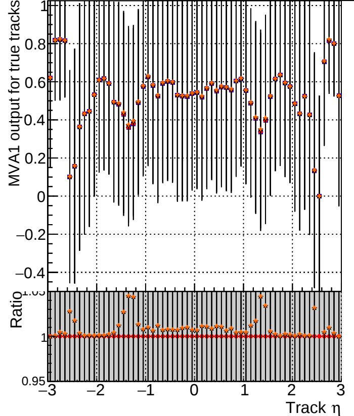
MVA1 of associated tracks (recoToSim) vs. track \eta Legend: ■ DQM_V0001_R0000000001 Global mkFit_original ● DQM_V0001_R0000000001 Global mkFit_pless ▲ DQM_V0001_R0000000001 Global mkFit_hptt ★ DQM_V0001_R0000000001 Global mkFit_new
