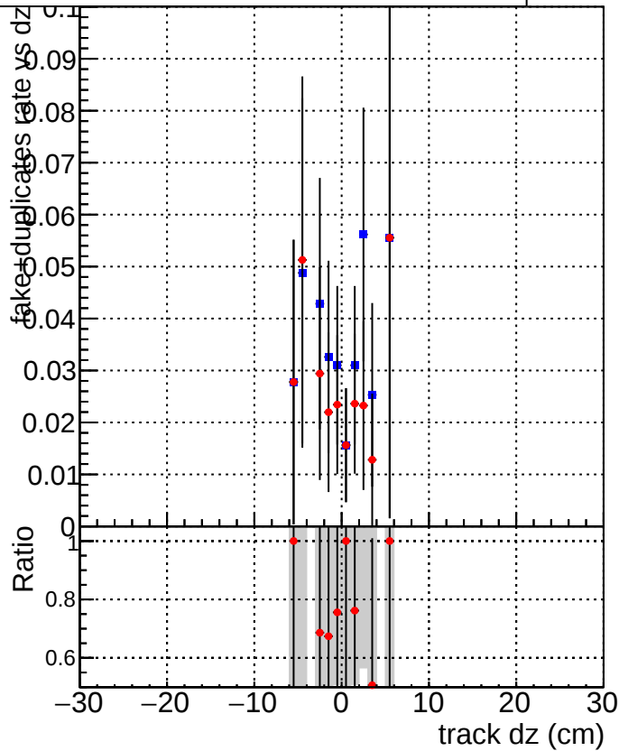
DQM_V0001_R000000001_Global_mkFit_original DQM_V0001_R000000001_Global_mkFit_pless
