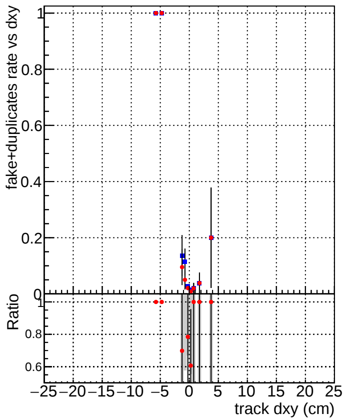
DQM_V0001_R000000001_Global_mkFit_original DQM_V0001_R000000001_Global_mkFit_pless
