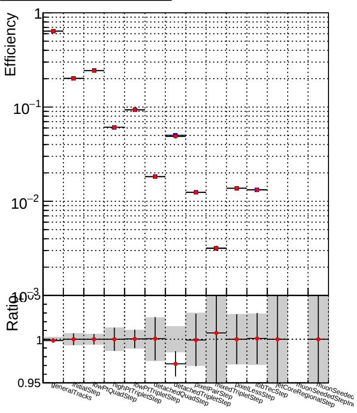
DQM_V0001_R000000001_Global_mkFit_original DQM_V0001_R000000001_Global_mkFit_det-triplet
