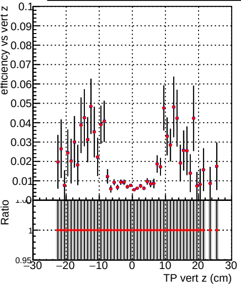
Efficiency vs vertpos Legend: DQM_V0001_R000000001_Global_mkFit_original DQM_V0001_R000000001_Global_mkFit_det-triplet
