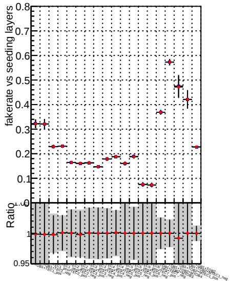
Fake rate vs. —•— DQM_V0001_R0000000001_Global_mkFit_original —•— DQM_V0001_R0000000001_Global_mkFit_def-triplet
