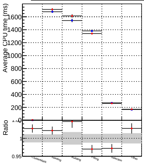
Average CPU time / built track
