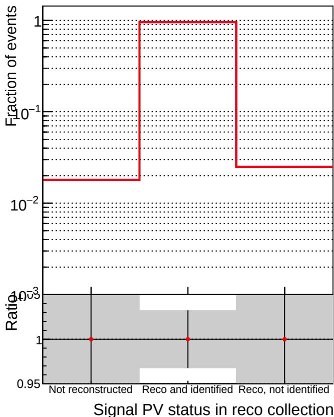
■ DQM_V0001_R000000001_Global_mkFit_original ● DQM_V0001_R000000001_Global_mkFit_det-triplet
