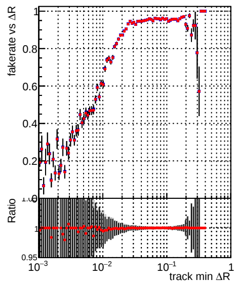
—•— DQM_V0001_R000000001_Global_mkFit_original —•— DQM_V0001_R000000001_Global_mkFit_det-triplet
