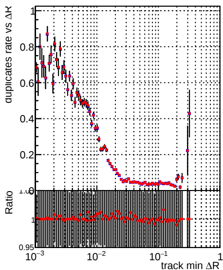
—•— DQM_V0001_R000000001_Global_mkFit_original —•— DQM_V0001_R000000001_Global_mkFit_det-triplet
