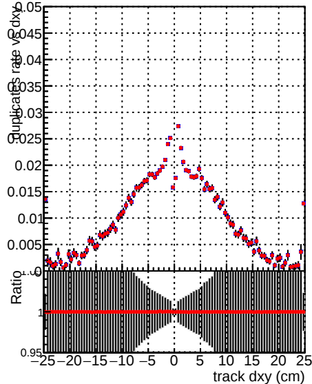
al__mkFit_det-triplet
