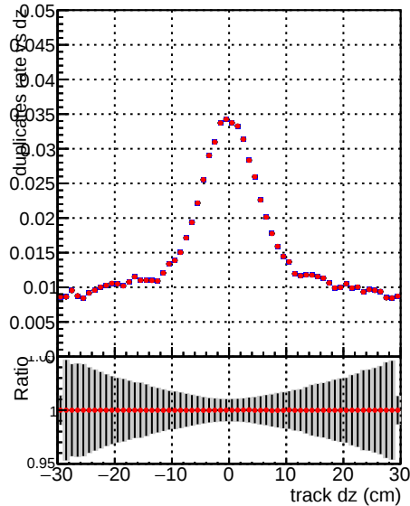
al__mkFit_det-triplet
