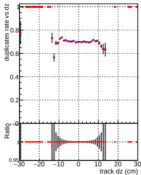
—●— DQM V0001_R000000001 Global mkFit original —●— DQM V0001_R000000001 Global mkFit det-triplet
