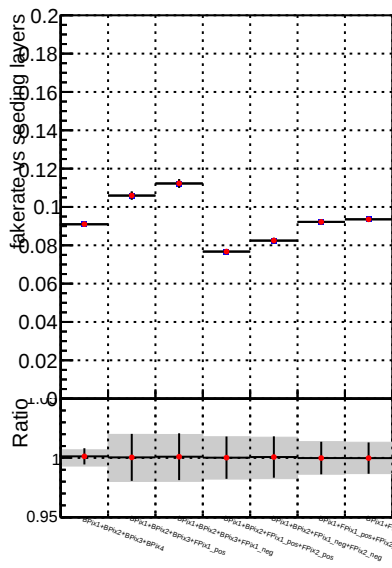
Fake rate vs. —•— DQM V0001_R000000001 Global mkFit original —•— DQM V0001_R000000001 Global mkFit def-triplet
