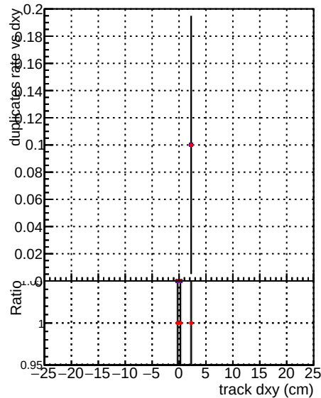
—•— DQM_V0001_R0000000001 Global mkFit original —•— DQM_V0001_R0000000001 Global mkFit def-triplet
