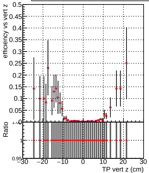
Efficiency vs. TP vert z (cm) — DQM_V0001_R000000001_Global_mkFit_original — DQM_V0001_R000000001_Global_mkFit_det-triplet
