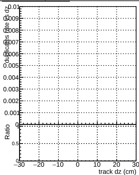
—•— DQM_V0001_R0000000001_Global_mkFit_original —•— DQM_V0001_R0000000001_Global_mkFit_def-triplet
