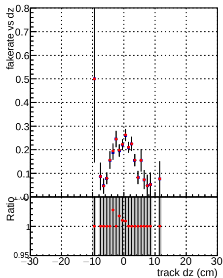
Fake rate vs dz —•— DQM_V0001_R0000000001_Global_mkFit_original —•— DQM_V0001_R0000000001_Global_mkFit_def-triplet
