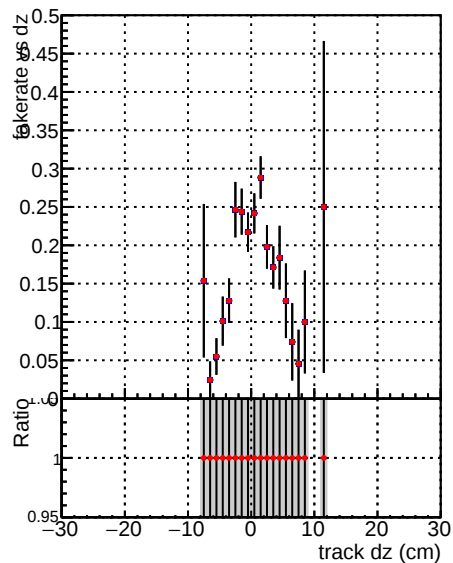
Fake rate vs dz Legend: Blue line with dots: DQM_V0001_R0000000001 Global mkFit original Red line with dots: DQM_V0001_R0000000001 Global mkFit det-triplet
