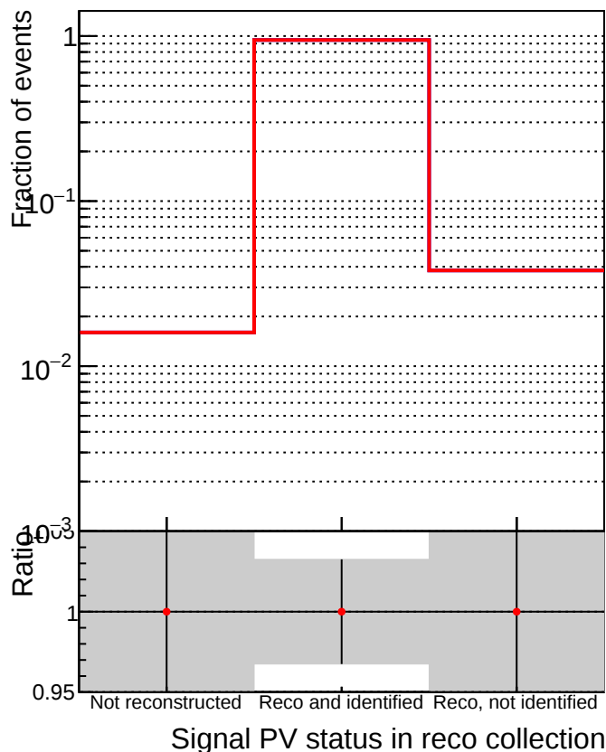
DQM_V0001_R000000001_Global_mkFit_original DQM_V0001_R000000001_Global_mkFit_det-triplet
