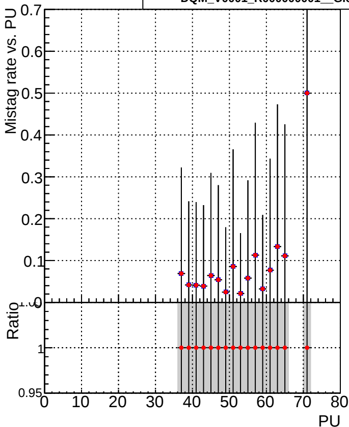
DQM_V0001_R000000001_Global_mkFit_original DQM_V0001_R000000001_Global_mkFit_det-triplet
