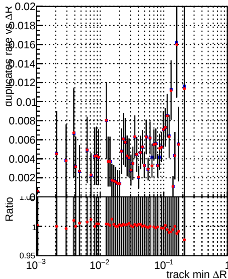
—●— DQM_V0001_R000000001_Global_mkFit_original —●— DQM_V0001_R000000001_Global_mkFit_det-triplet
