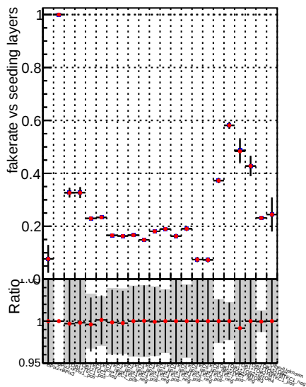
Fake rate vs. Legend Global mkFit Blue line with dots DQM_V0001_R0000000001 original Red line with dots DQM_V0001_R0000000001 def-triplet
