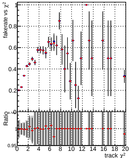
Fake rate vs. Legend Global mkFit original Blue diamond DQM_V0001_R0000000001 Global Red diamond DQM_V0001_R0000000001 mkFit def-triplet
