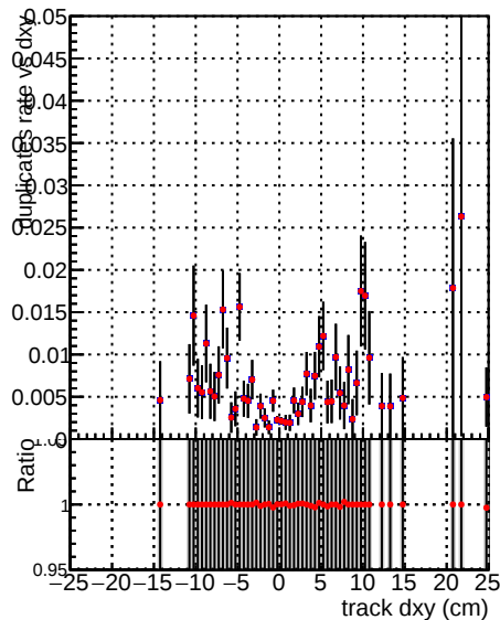
—●— DQM_V0001_R0000000001 Global mkFit_original —●— DQM_V0001_R0000000001 Global mkFit_def-triplet
