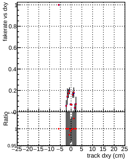
—•— DQM_V0001_R0000000001_Global_mkFit_original —•— DQM_V0001_R0000000001_Global_mkFit_def-triplet
