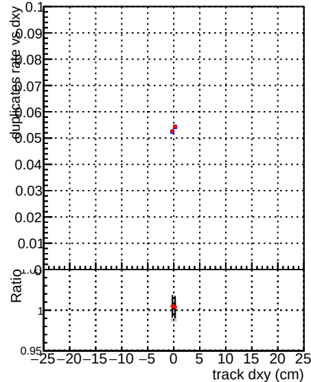
al_mkFitQCdi1_RECO al_mkFitQCDmod_RECO
