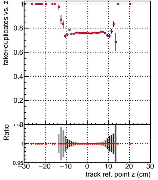
■ DQM_V0001_R000000001_Global_mkFitQCDi1_RECO ◆ DQM_V0001_R000000001_Global_mkFitQCDmod_RECO
