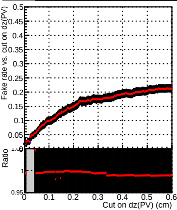
Fake rate Legend: DQM_V0001_R000000001_Global_mkFitQCDi1_RECO DQM_V0001_R000000001_Global_mkFitQCDmod_RECO
