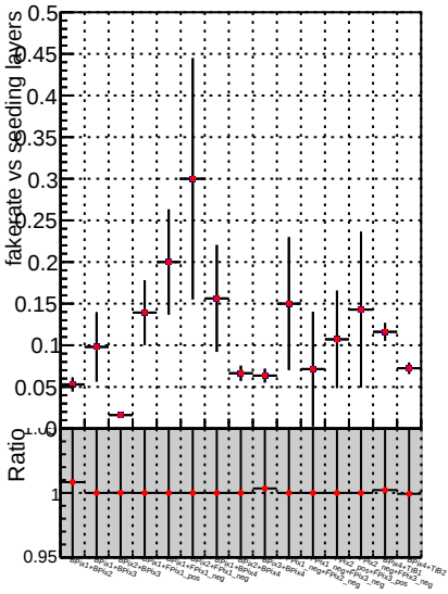
Fake rate vs. — DQM_V0001_R0000000001_Global_mkFitQCDi1_RECO — DQM_V0001_R0000000001_Global_mkFitQCDmod_RECO
