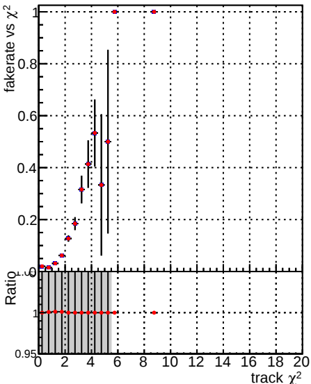
Fake rate vs. — DQM_V0001_R0000000001_Global_mkFitQCDi1_RECO — DQM_V0001_R0000000001_Global_mkFitQCDmod_RECO
