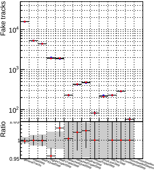
Number —●— DQM_V0001_R0000000001_Global_mkFitQCDmod_RECO
