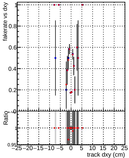
—●— DQM_V0001_R0000000001_Global_mkFitQCDi1_RECO —●— DQM_V0001_R0000000001_Global_mkFitQCDmod_RECO
