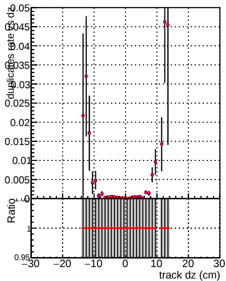
—●— DQM_V0001_R0000000001_Global_mkFitQCDi1_RECO —●— DQM_V0001_R0000000001_Global_mkFitQCDmod_RECO
