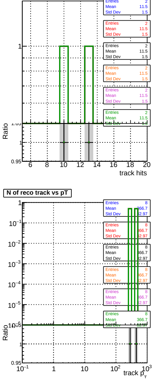
N of reco track vs pT
