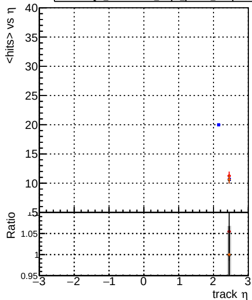
mean hit DQM_original4_step2_pt1000_eta2p0to2p5 DQM_testMkFit_step2_pt1000_eta2p0to2p5 DQM_testMkFitFit_step2_pt1000_eta2p0to2p5 DQM_testMkFitFit_step2_pt1000_eta2p0to2p5_Rej10
