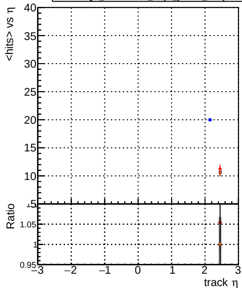
DQM_original4_step2_pt1000_eta2p0to2p5 DQM_testMkFit_step2_pt1000_eta2p0to2p5 DQM_testMkFitFit_step2_pt1000_eta2p0to2p5 DQM_testMkFitFit_step2_pt1000_eta2p0to2p5_Rej10
