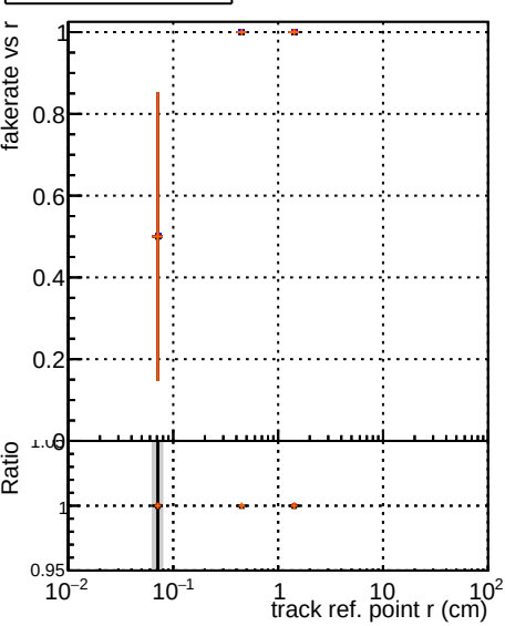
DOM original4 step2 pt1000 eta2p0to2p5 DOM test5MKFit step2 pt1000 eta2p0to2p5 DOM test5MKFit step2 pt1000 eta2p0to2p5 DOM test5MKFit step2 pt1000 eta2p0to2p5 Rej10
