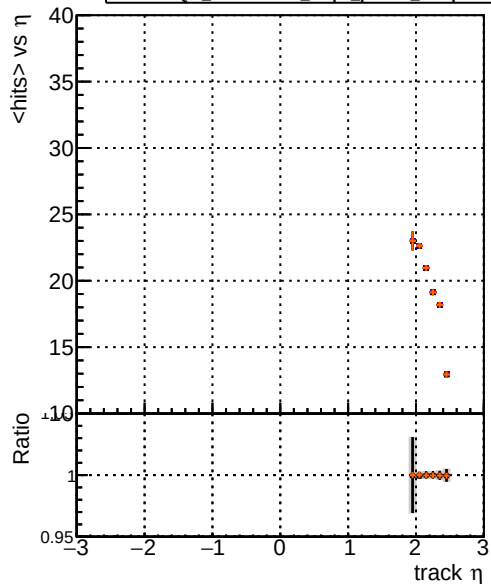
mean hits vs \eta DQM_original4_step2_pt1000_eta2p0to2p5 DQM_testMkFit_step2_pt1000_eta2p0to2p5 DQM_testMkFitFit_step2_pt1000_eta2p0to2p5 DQM_testMkFitFit_step2_pt1000_eta2p0to2p5_Rej10
