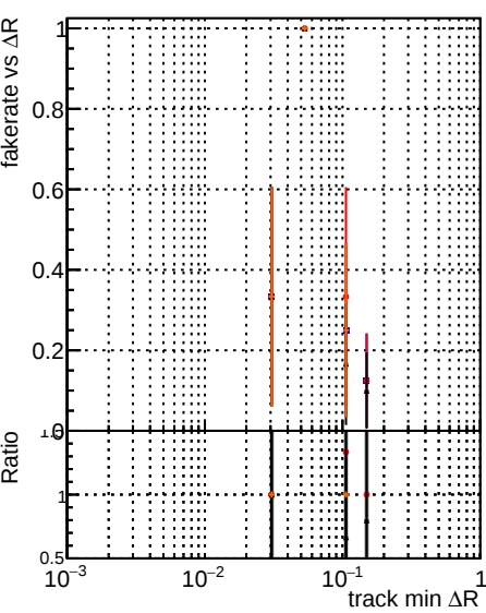
Fake rate vs \Delta R(\text{track}, \text{jet}) Legend: DOM original4_step2_pt1000_eta2p0to2p5, DOM testIMKFit_step2_pt1000_eta2p0to2p5, DOM testIMKFit_step2_pt1000_eta2p0to2p5_Rej10
