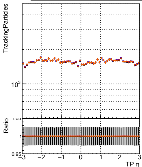
● DQM_original14 ● DQM_testMkFit_initialStepReso ● DQM_testMkFitFit_initialStepReso ● DQM_testMkFitFit_initialStepReso_wRejection25
