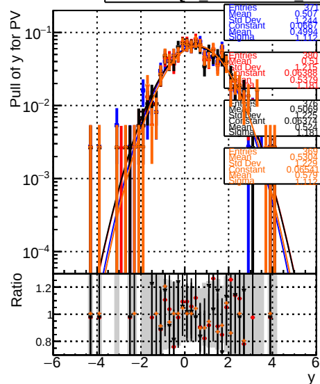
RecoPVAssoc2GenPVMatched_PullY Legend: DOM original, DOM initialStepReso, DOM initialStepReso wRejection25, DOM initialStepReso
