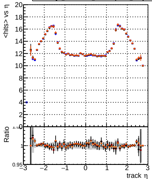
mean hit DQM_original4 DQM_testMkFit_initialStepReso DQM_testMkFitFit_initialStepReso DQM_testMkFitFit_initialStepReso_wRejection25
