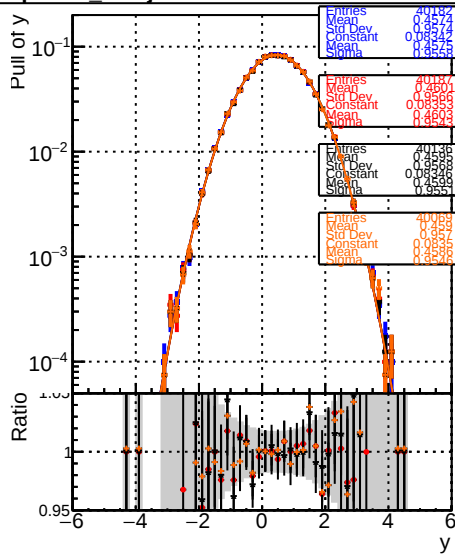
RecoAllAssoc2GenMatched_PullY
