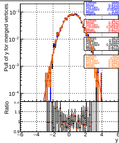
RecoAllAssoc2GenMatchedMerged_PullY
