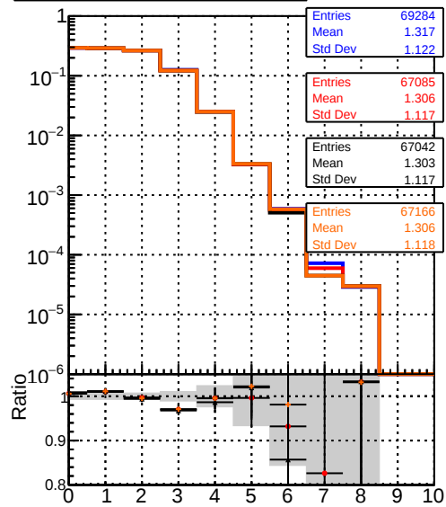
DQM_original4 DQM_testMkFit_fit_initialStepReso DQM_testMkFitFit_initialStepReso DQM_testMkFitFit_initialStepReso_wRejection25 mean hit
